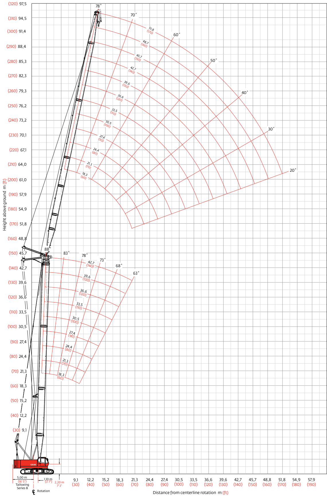
No. 12000 luffing jib on luffing boom
