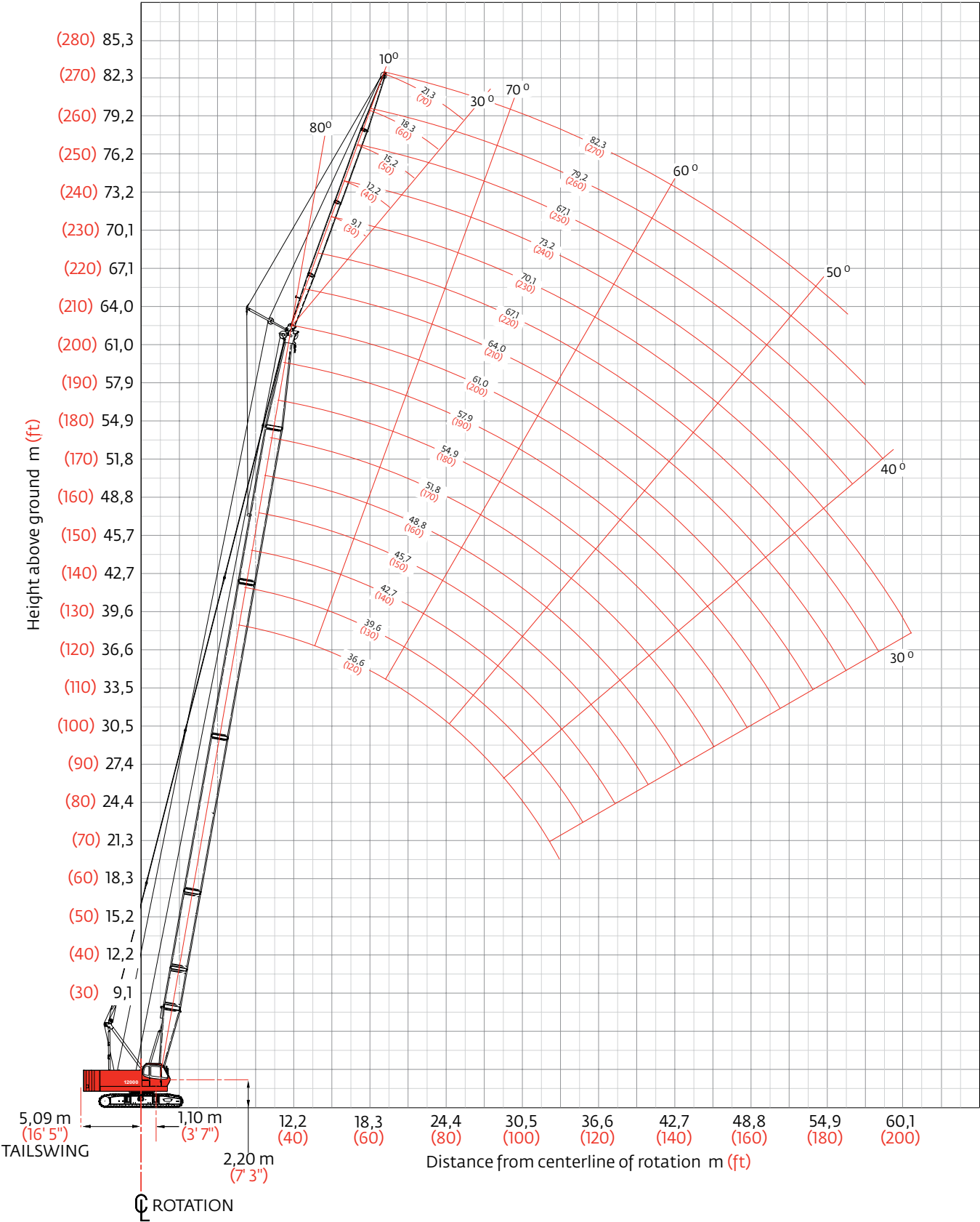
No. 12000 fixed jib on main boom
