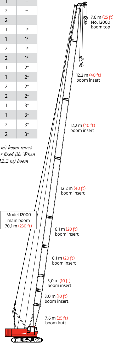
Model 12000 Main boom 70,1 m (230 ft)
