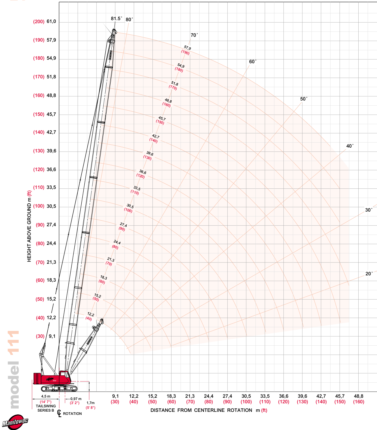
No. 111 Main Boom
