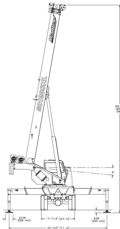
FULL SPREAD
