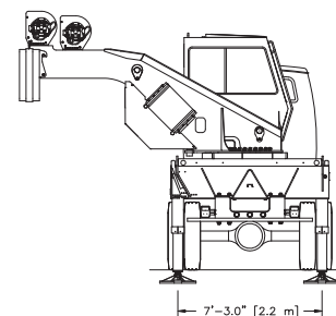
RETRACTED SPREAD
