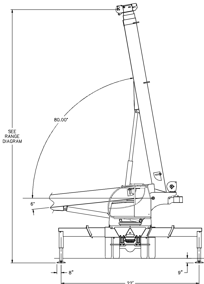
Full Extension
