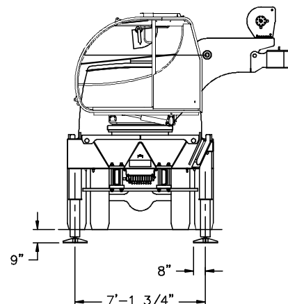
Full Retraction
