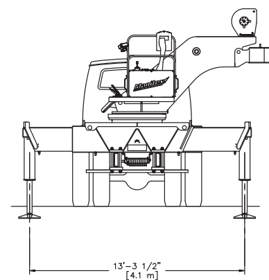
INTERMEDIATE SPREAD
