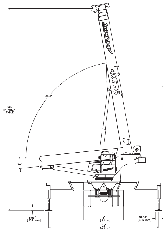
FULL SPREAD
