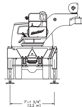
RETRACTED SPREAD
