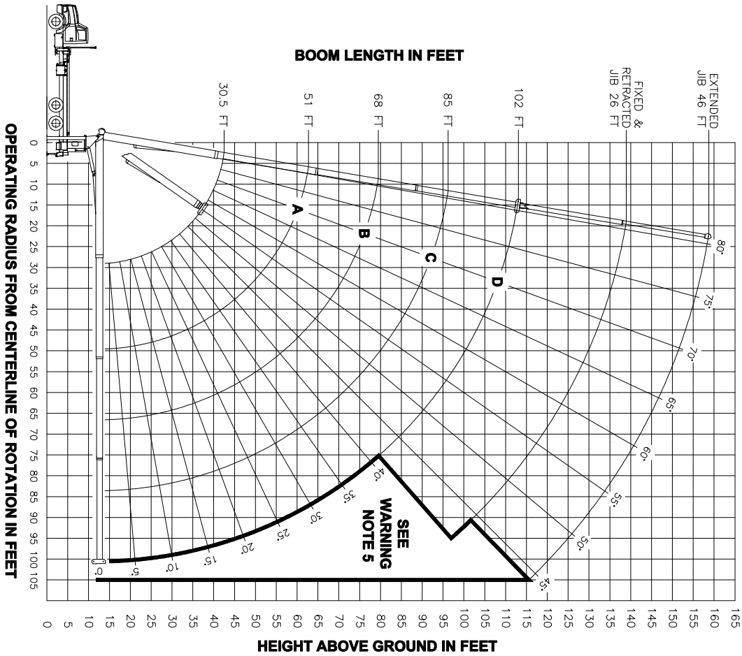
RANGE DIAGRAM
