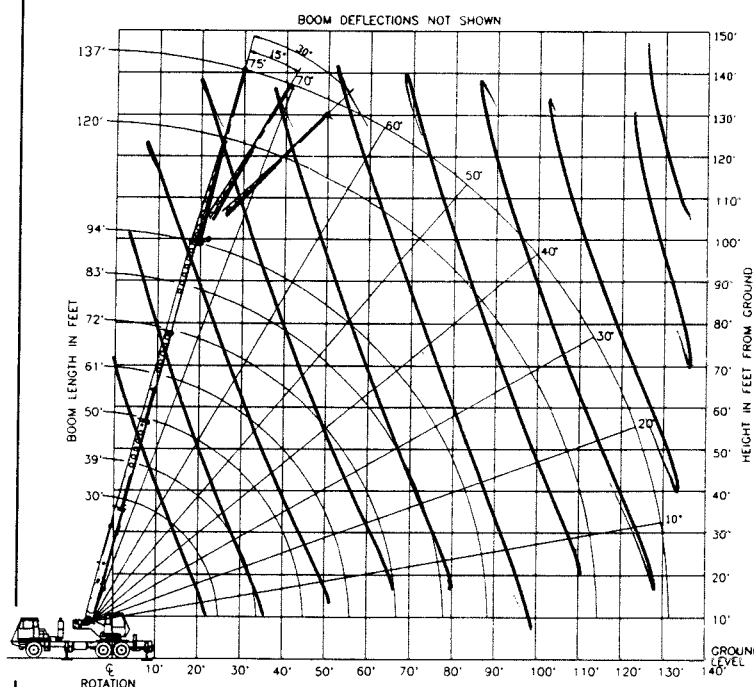
Range Diagram (30' - 94' boom)
