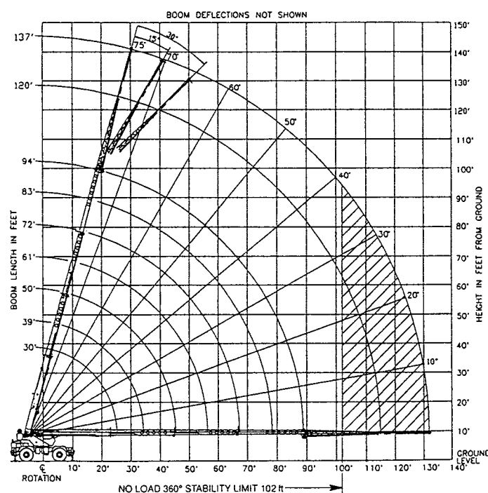
Range Diagram (30' - 94' boom)
