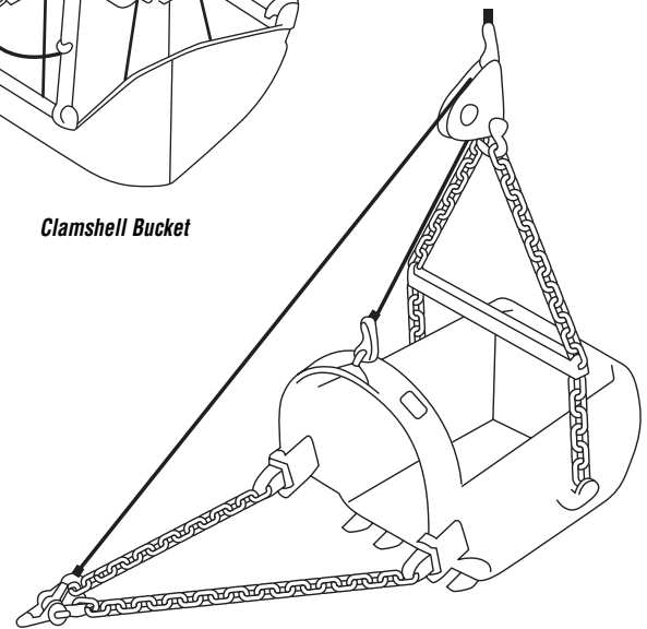
Dragline Bucket
