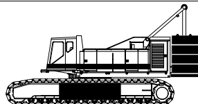
Main Boom Capacities – 300 Ft. – Open Throat Boom
