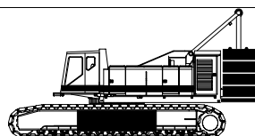
Main Boom Capacities – 100 Ft. – Open Throat Boom
