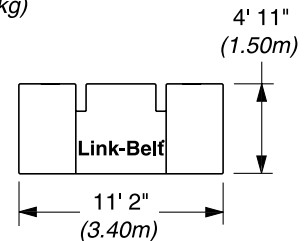
"B" Upper Counterweight 22,500 lbs. (10 206 kg)
