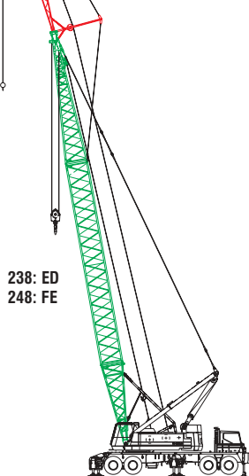
Boom and jib - open throat
