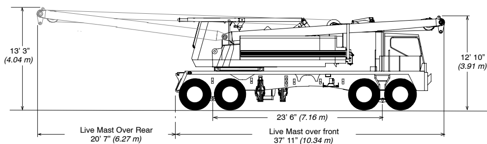
Axle weights Live Mast, without pusher axle and without front or rear O/R box. (Includes ropes and standard backstops)
