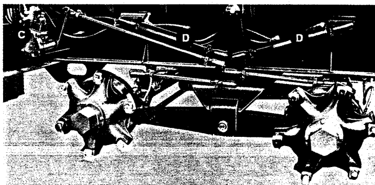
Power assist hydraulic steer
