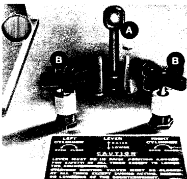
Counterweight lowering/raising control
