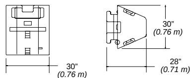
#7 Counterweight (two) – 3,968 lbs. (1 800 kg) – each
