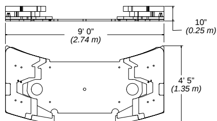
#2, 3, & 4 Counterweights – 5,512 lbs. (2 500 kg)
