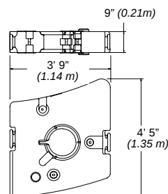
#8 Counterweight (two) – 4,409 lbs. (2 000 kg) – each
