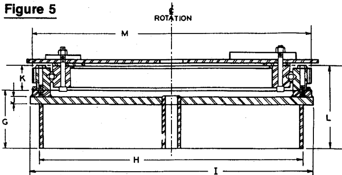
Models 138, 218 & 238
