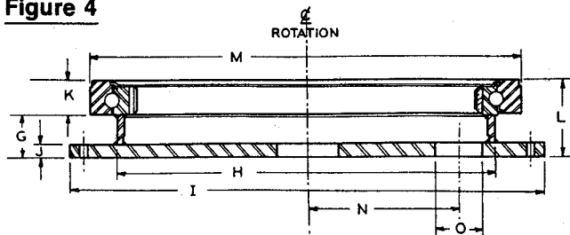
Model 48A
