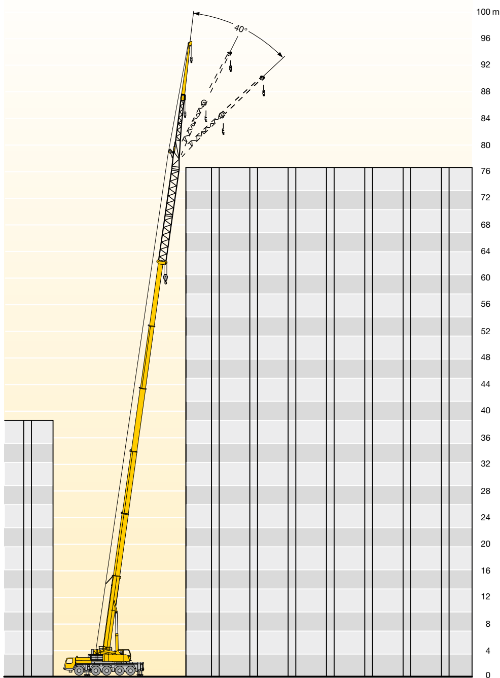
Hydraulically adjustable folding jib (0° to 40°)
