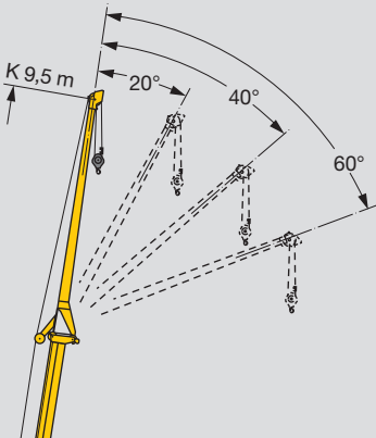
9.5 m long swing-away jib adjustable up to 60°
