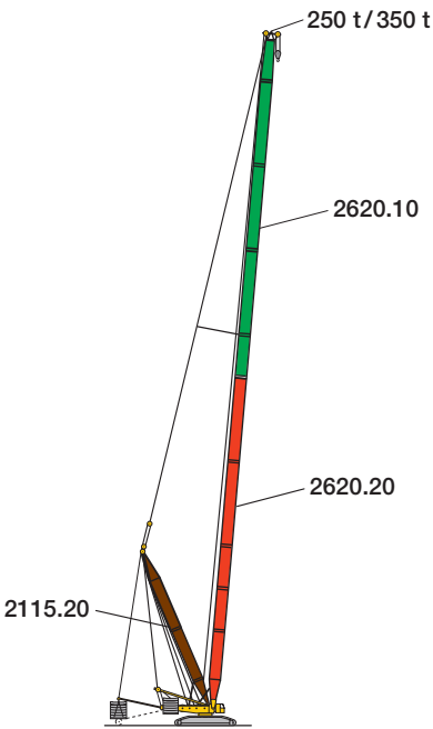
SLD/SLDB/BW SL 28 m – 112 m D 21 m – 28 m
