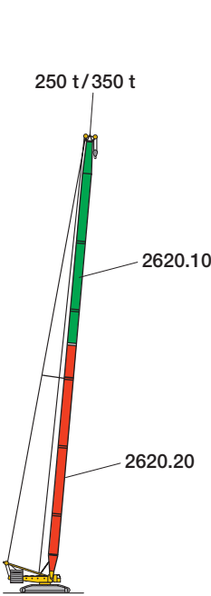
SL SL 21 m – 91 m
