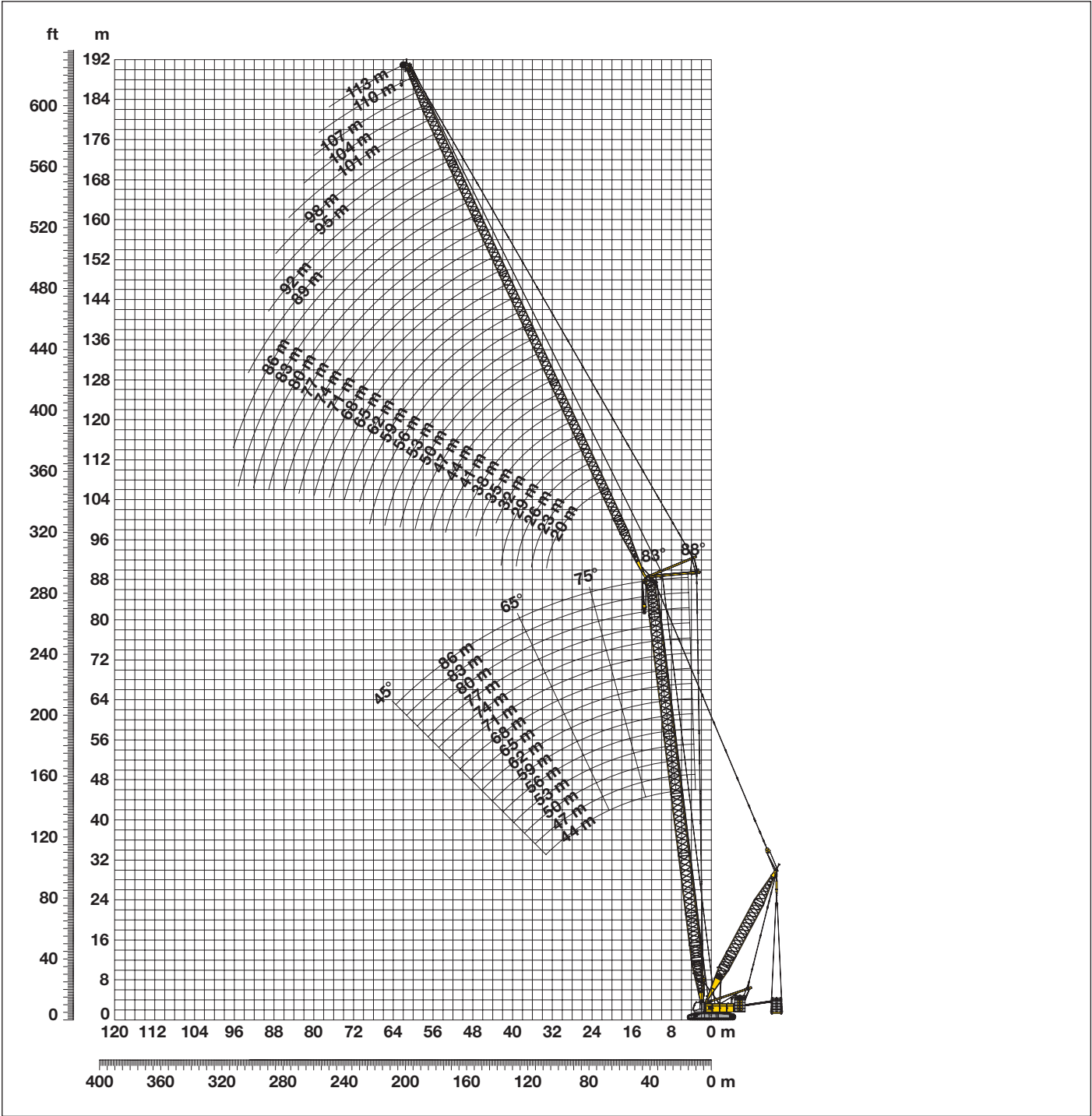
Boom configuration for main boom lengths (44 m - 86 m) – see table 1 on page 4 Jib configuration for jib lengths (20 m - 113 m)
