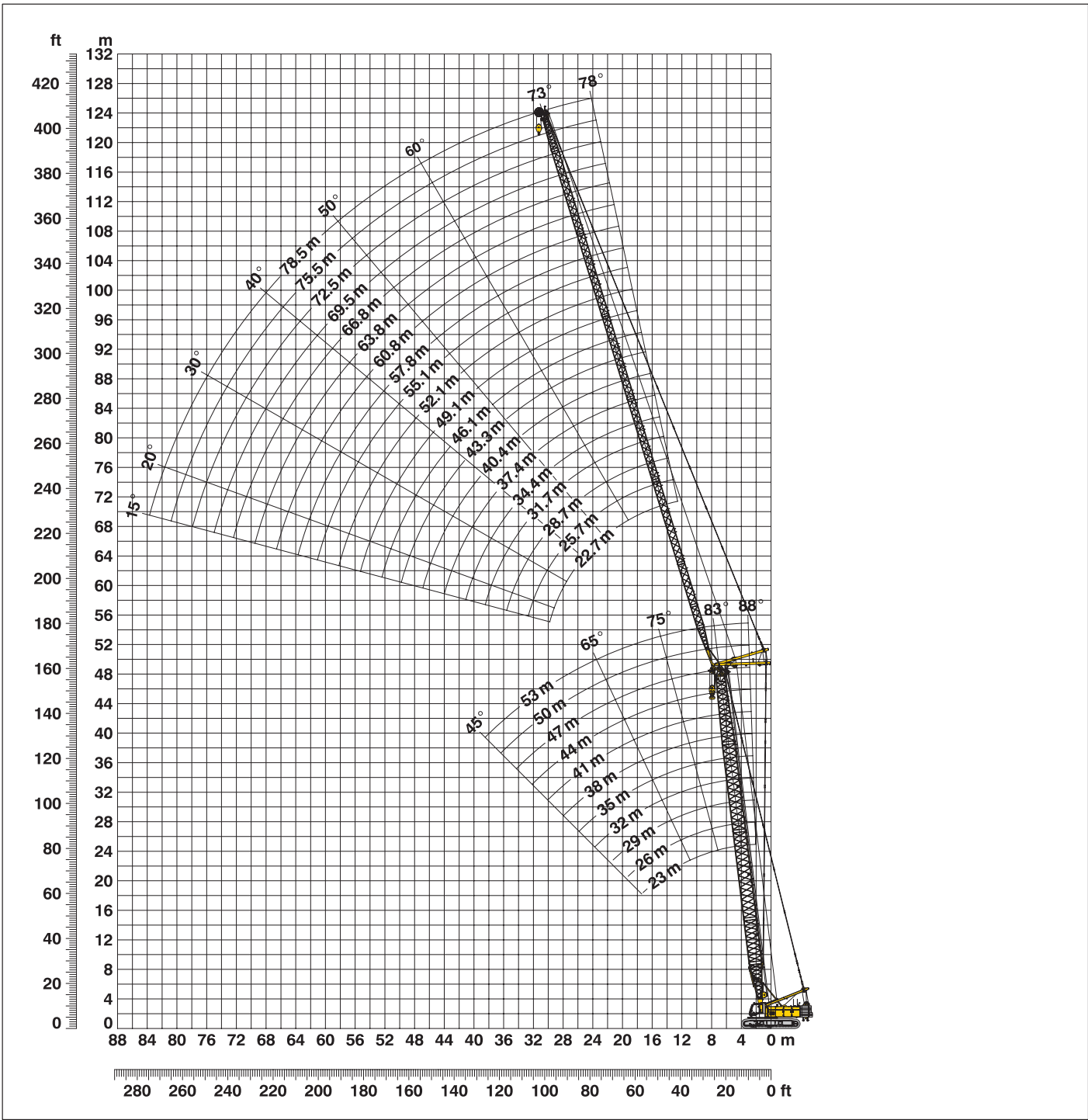
Boom configuration for main boom lengths (23 m - 53 m) – see table 1 on page 10 Jib configuration for jib lengths (22.7 m - 78.5 m)
