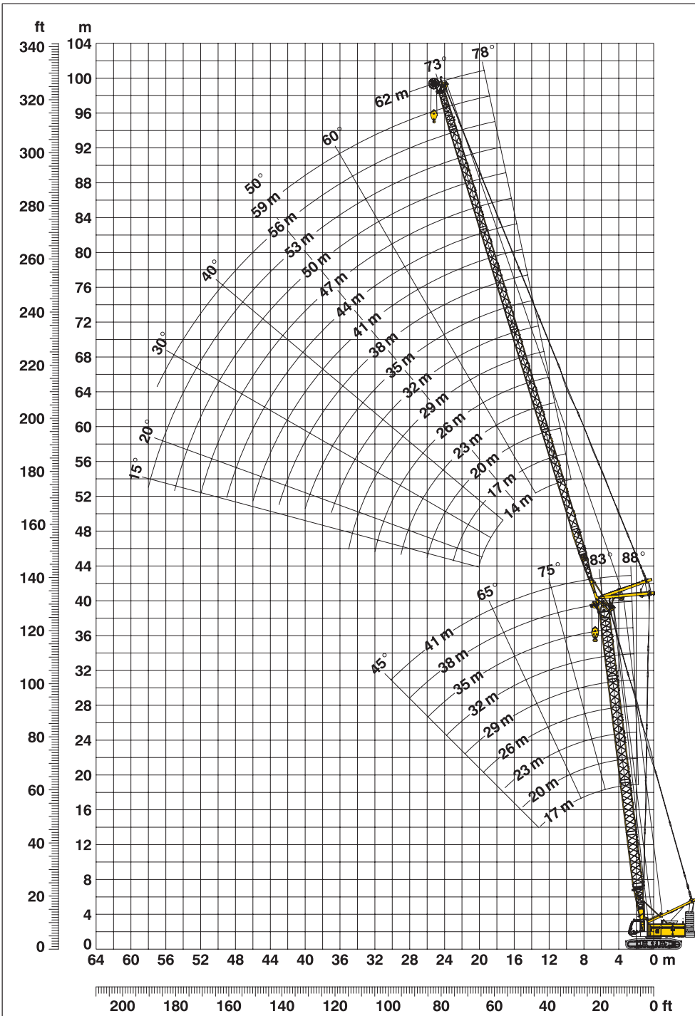
Boom configuration for main boom lengths (17 m - 41 m) – see table 1 on page 12 Jib configuration for jib lengths (14 m - 62 m)
