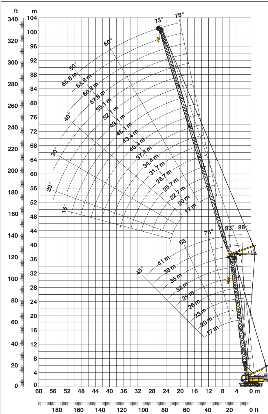
Boom configuration for main boom lengths (17 m - 41 m) – see table 1 on page 12 Jib configuration for jib lengths (17 m - 66.8 m)
