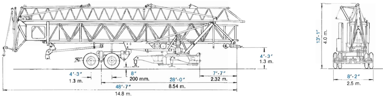
Transporter (Fifth wheel unit without counterweights)
