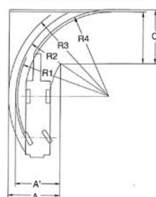
2-Drive Steering (Rear)
