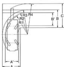
4-Drive Steering
