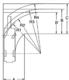
2-Drive Steering (Front)
