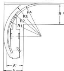
2-Drive Steering (Rear)
