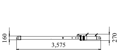
Strut Backstop (Luffing Jib) Weight: 180 kg
