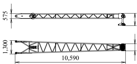
Front Strut (Luffing Jib) Weight: 1,410 kg
