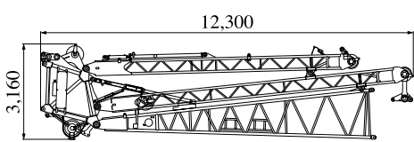
Travel Kit Assembly Weight: 6,730 kg
