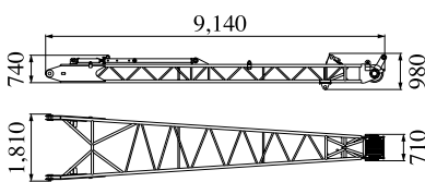
Rear Strut (Luffing Jib) Weight: 1,510 kg
