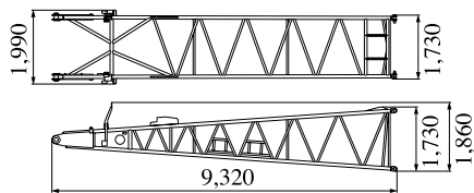
Luffing Jib Base Weight: 1,470 kg
