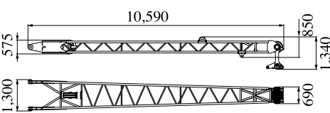
Front Strut (Luffing Jib) Weight: 1,410 kg
