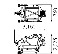
Luffing Boom Top Weight: 2,085 kg
