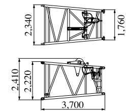
Luffing Tapered Boom Weight: 1,190 kg
