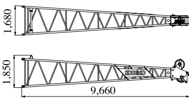
Luffing Jib Top Weight: 1,400 kg
