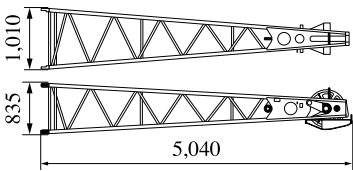
Jib Top (For Crane) Weight: 315 kg
