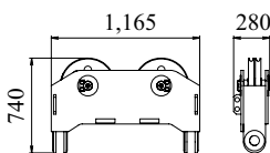
Lower Spreader (for Crane) Weight: 300 kg
