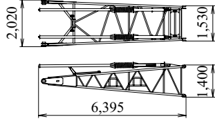
Jib Tip (Luffing Jib) Weight: 1,170 kg
