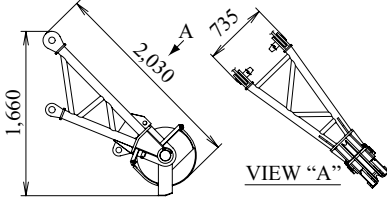
Auxiliary Sheave (for Crane) Weight: 300 kg
