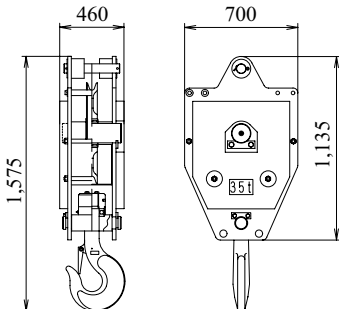
35 t Hook Weight: 900 kg
