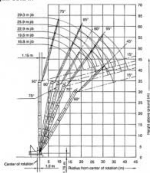
Tower Length: 36.3 m
