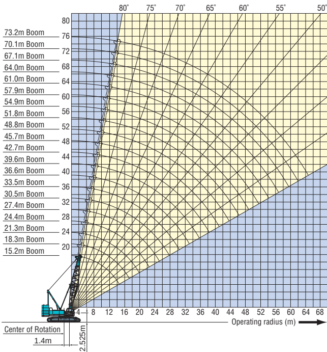
Heavy-duty Boom Working Range
