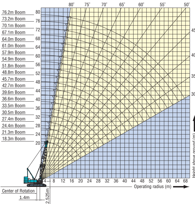
Light-duty Boom Working Range
