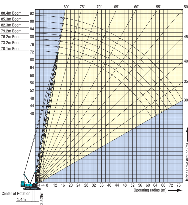
Long Boom Working Range
