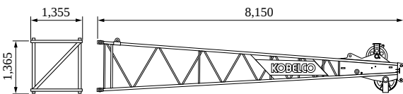
Jib Top (for Luffing Tower) Weight: 900 kg
