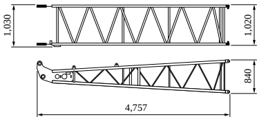
Jib Base (For Crane) Weight: 210 kg
