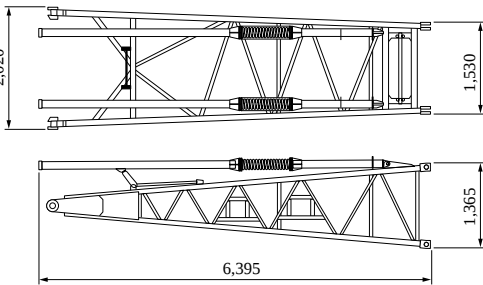
Jib Base (for Luffing Tower) Weight: 1,200 kg
