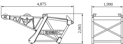
Luffing Tower Cap Weight: 1,780 kg
