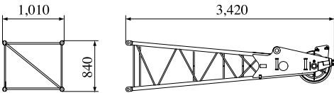
Tower Jib Top Weight: 245 kg
