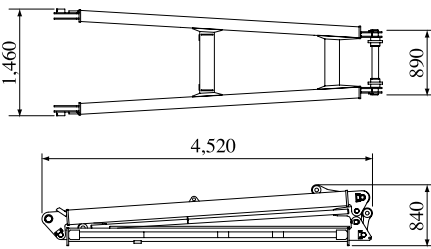
Tower Jib strut Weight: 760 kg
