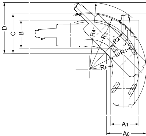
●Left turn in 4-wheel steering mode
