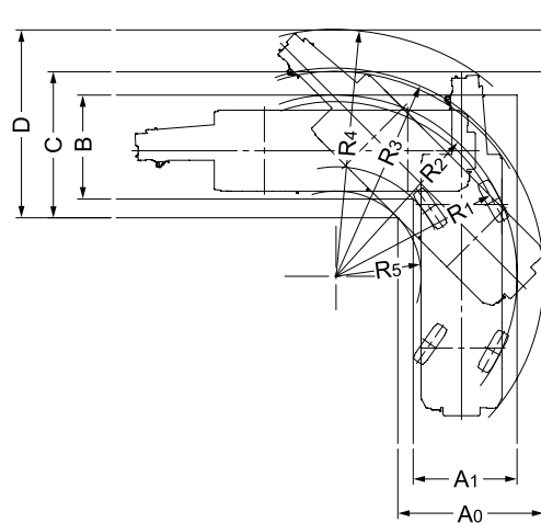
●Left turn in 4-wheel steering mode
