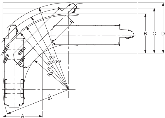
●Right turn in 4-wheel steering mode
