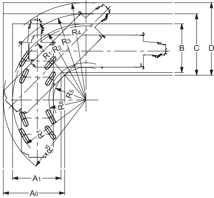
●Right turn in 8-wheel steering mode
