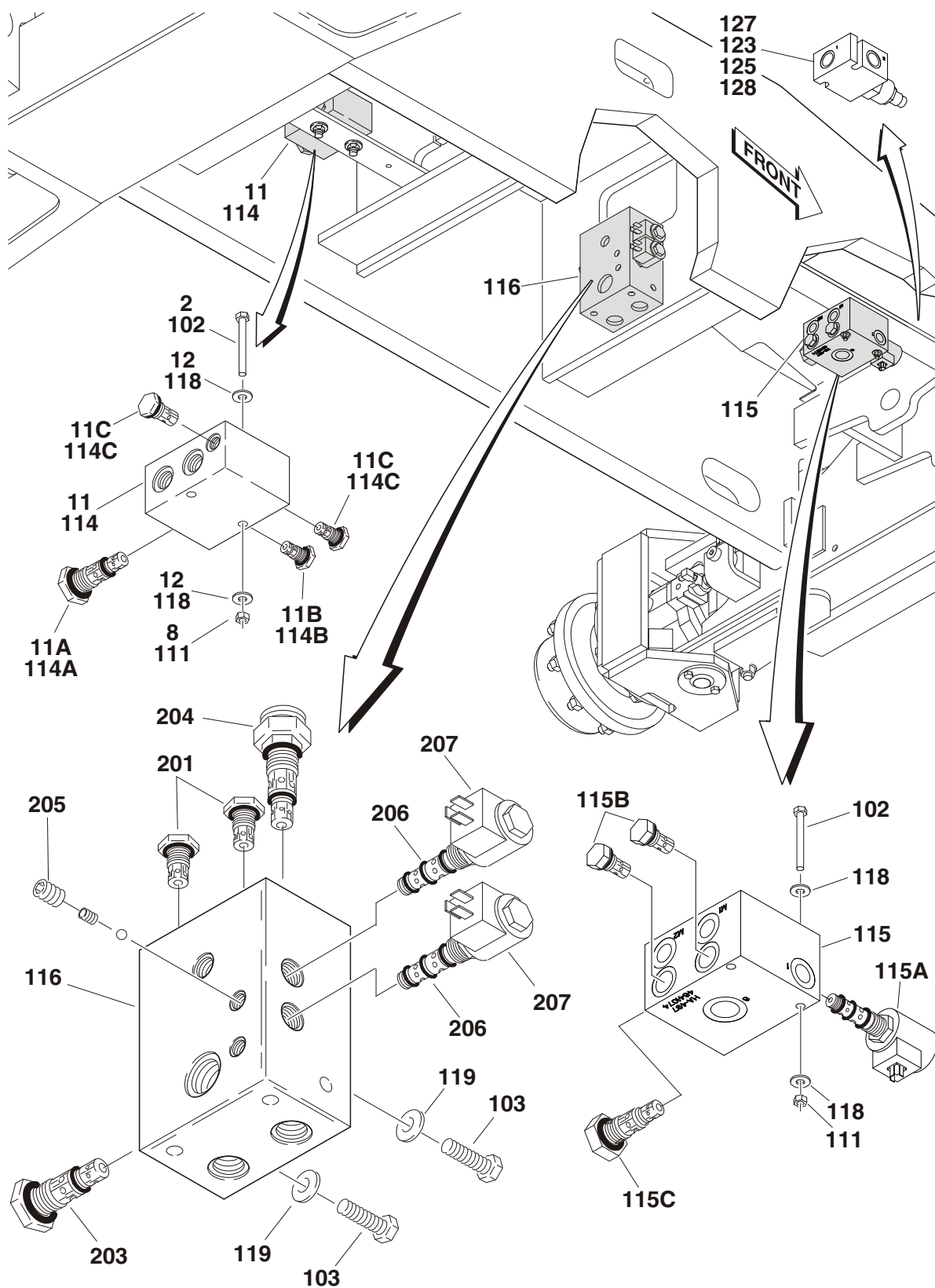
FIGURE 1-10. DRIVE VALVES INSTALLATIONS
