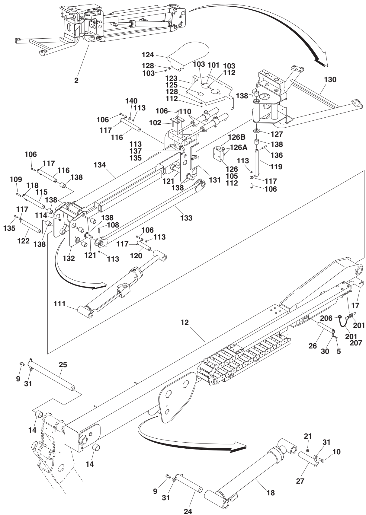
FIGURE 3-3. MAIN BOOM AND CYLINDERS INSTALLATION - 450AJ
