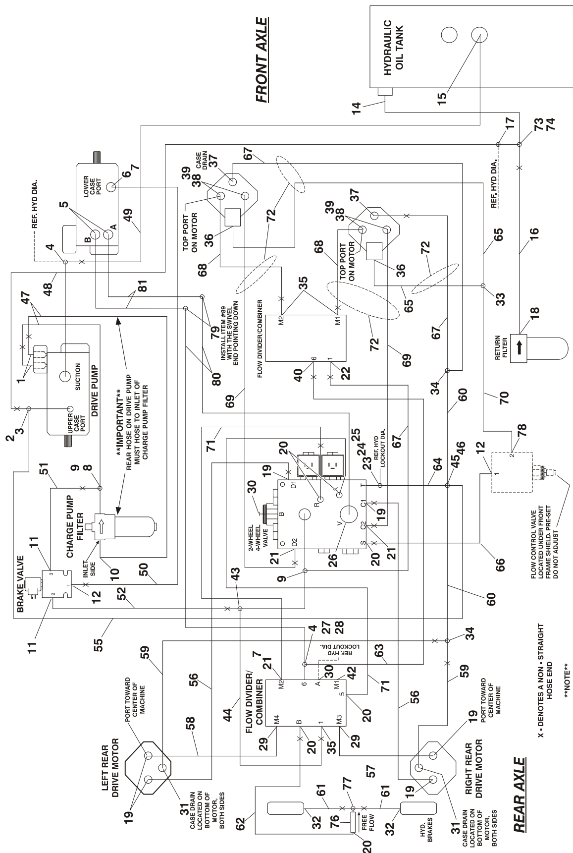
FIGURE 6-5.DRIVE HYDRAULIC DIAGRAM - 4WD
