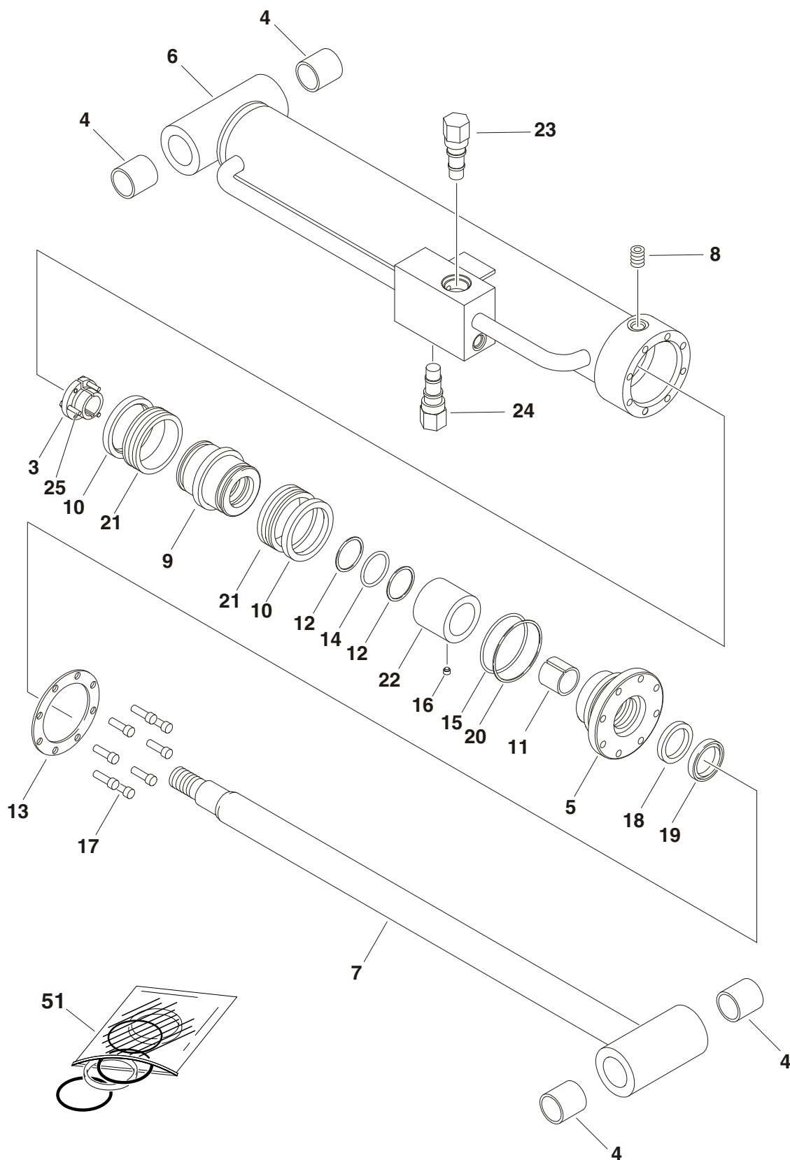
FIGURE 5-3. LIFT CYLINDER ASSEMBLY - JIB (450AJ ONLY)
