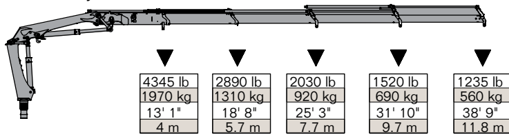
9/65DL - 4 Hydraulic
