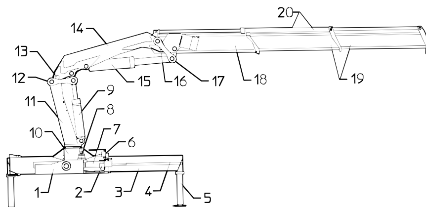
FIGURE 1:LOADER OVERVIEW
