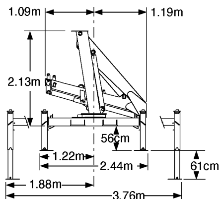
STOWED POSITION AND OUTRIGGER DIMENSIONS (1 HYD EXTENSION)
