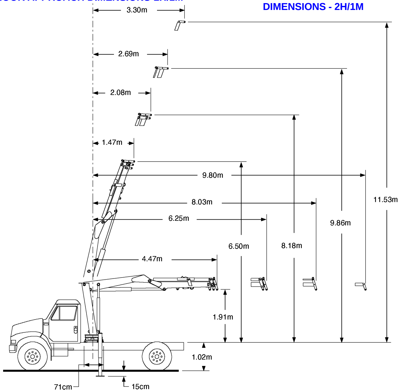
GEOMETRIC CONFIGURATION-2HYD & 2HYD/1MNL EXTENSIONS-MODEL 780 CRANE
