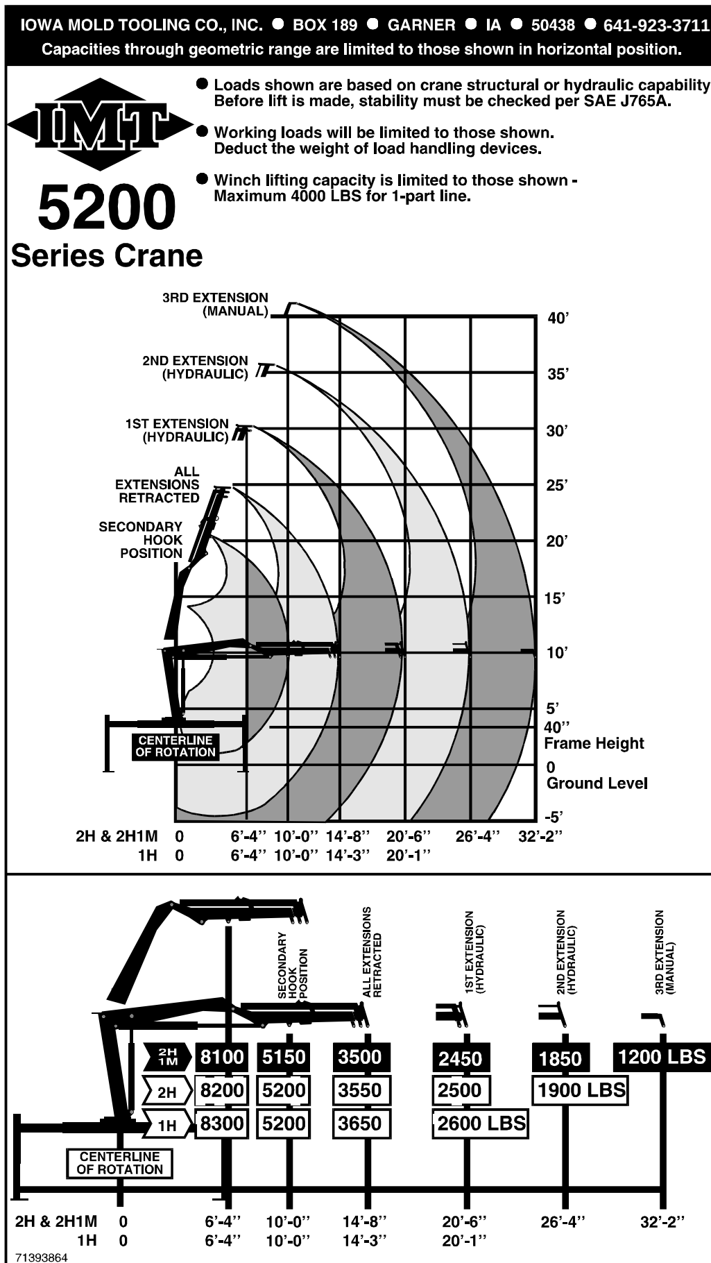
CAPACITY CHART-5200 SERIES CRANE
