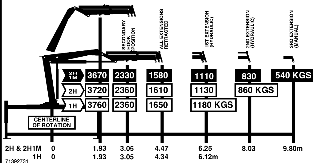
CAPACITY CHART-MODEL 780 CRANE
