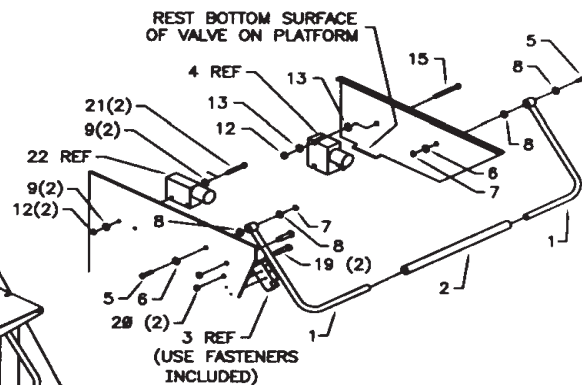
EXPLODED ASSEMBLY
