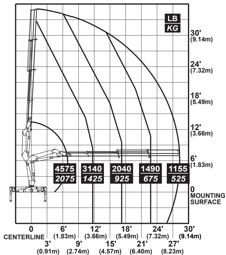
3-Hydraulic
