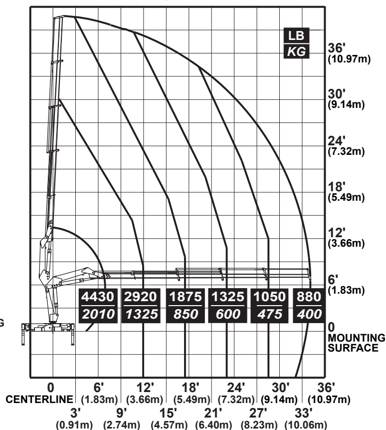
4-Hydraulic
