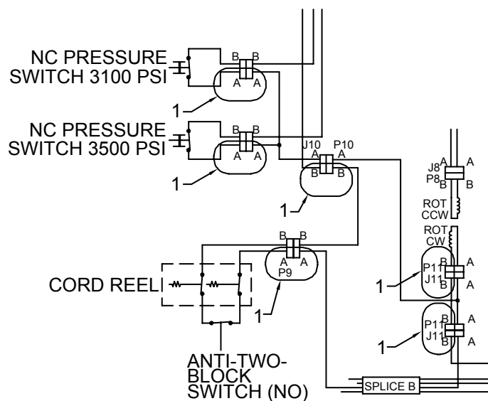
ANTI-TWO-BLOCK ASSEMBLY
