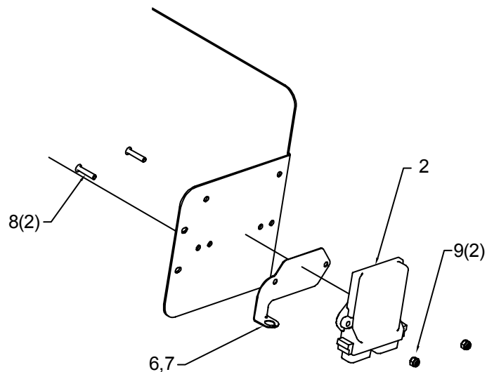
RECEIVER ASSEMBLY DETAIL
