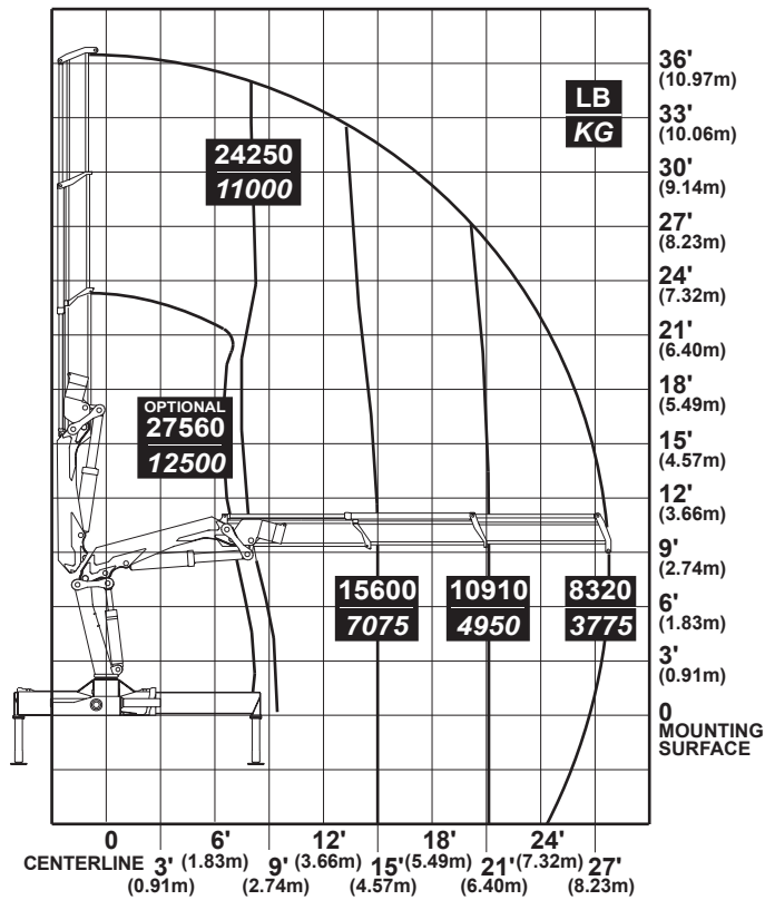
2-Hydraulic
