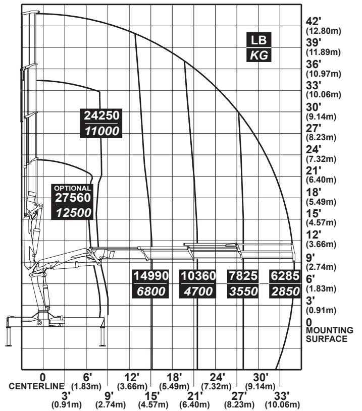
3-Hydraulic
