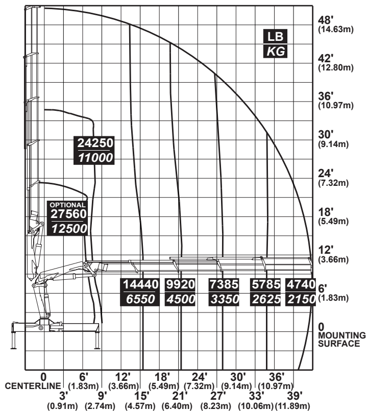
4-Hydraulic
