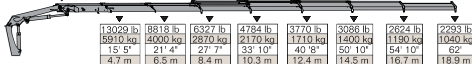
32/222 - 8 Hydraulic
