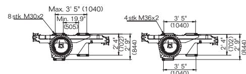
(EXTRA VALVES, K2-K6) (EXTRA VALVES, K7-K8)
