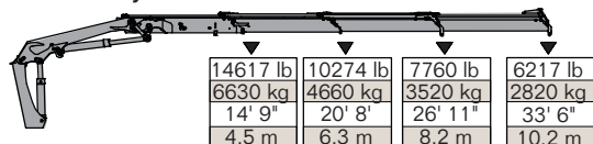
32/222 - 3 Hydraulic
