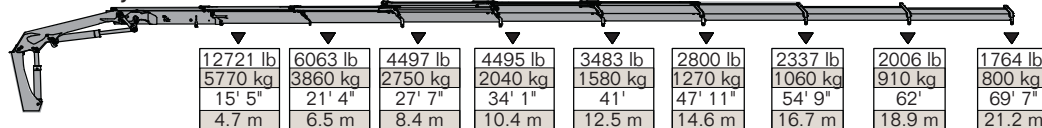
32/222 - 8 Hydraulic
