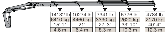
32/222 - 4 Hydraulic
