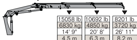
32/222 - 2 Hydraulic
