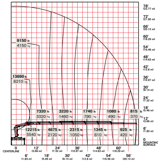
20/138DL K8
