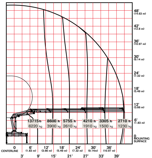
20/138SL K4
