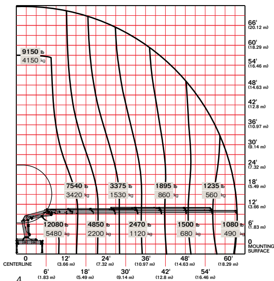
20/138SL K7
