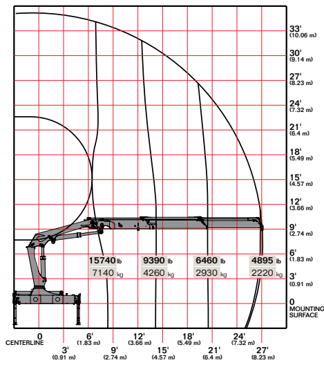
20/138DL K2
