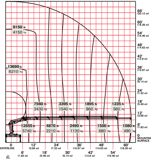
20/138DL K7
