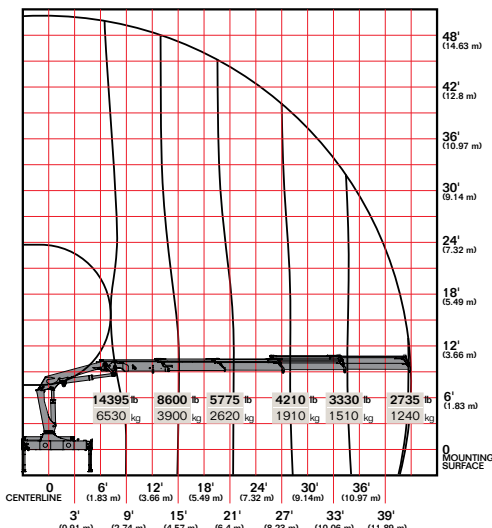
20/138DL K4
