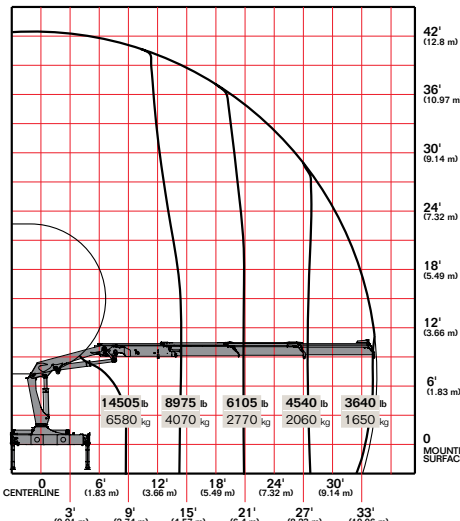
20/138SL K3
