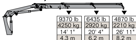
20/138SL - 2 Hydraulic
