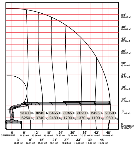
20/138DL K7
