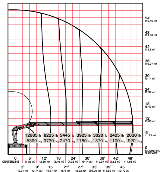
20/138SL K5
