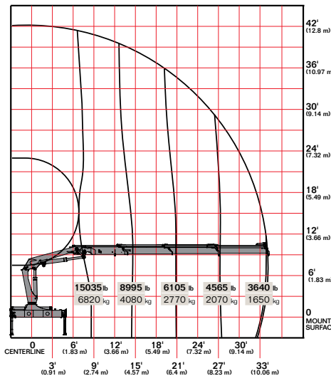
20/138DL K3
