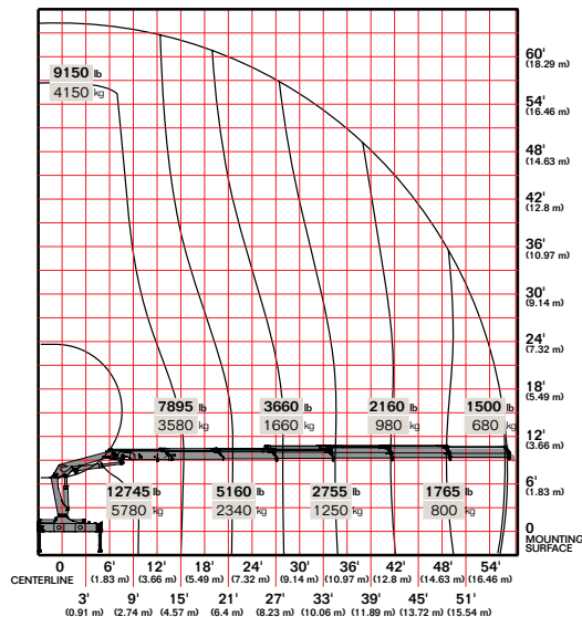
20/138SL K6
