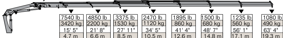
20/138SL - 8 Hydraulic
