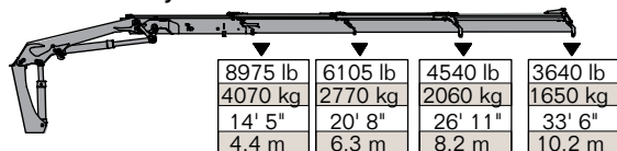
20/138SL - 3 Hydraulic
