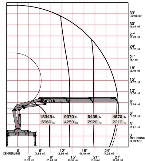
20/138SL K2
