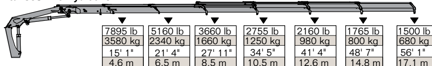
20/138SL - 6 Hydraulic
