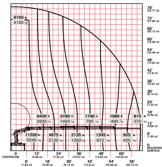
20/138SL K8
