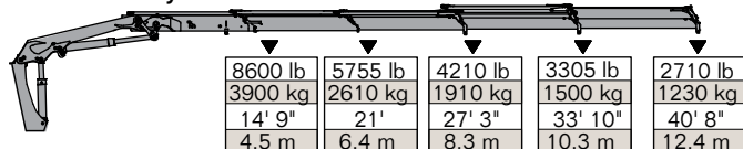
20/138SL - 4 Hydraulic
