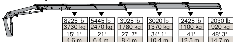
20/138SL - 5 Hydraulic
