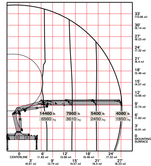
17/117DL K2
