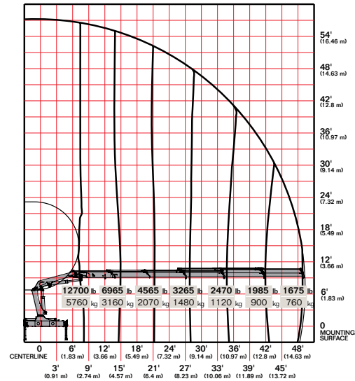
17/117DL K5
