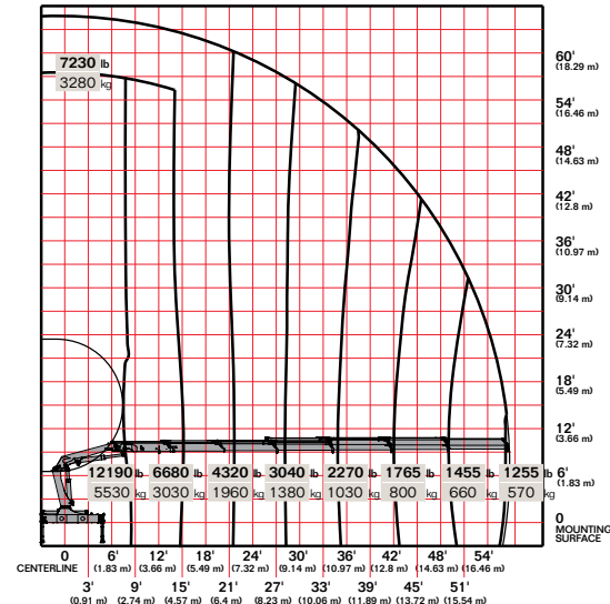
17/117DL K6
