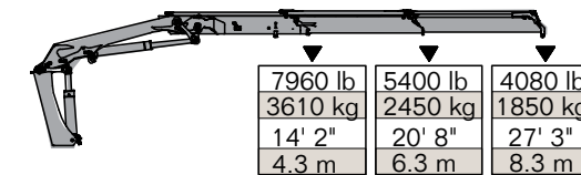
17/117DL - 2 Hydraulic
