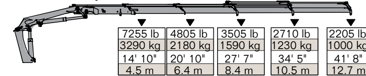
17/117DL - 4 Hydraulic
