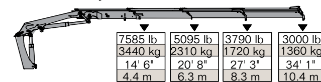
17/117DL - 3 Hydraulic
