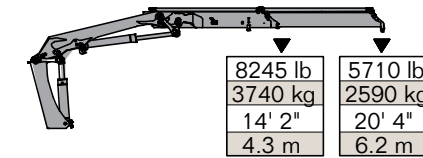
17/117DL - 1 Hydraulic
