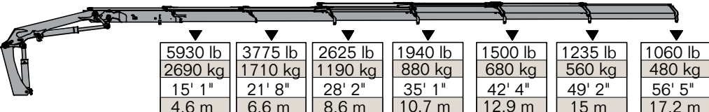
15/105DL - 6 Hydraulic
