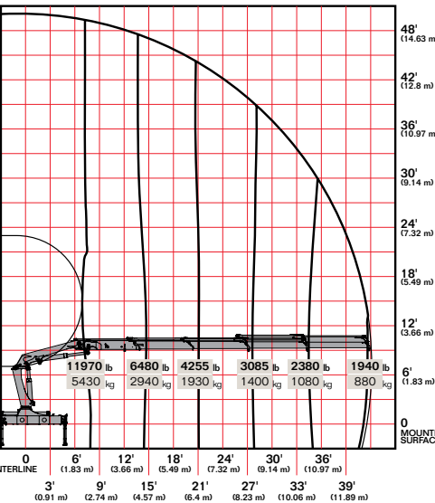
15/105DL K6
