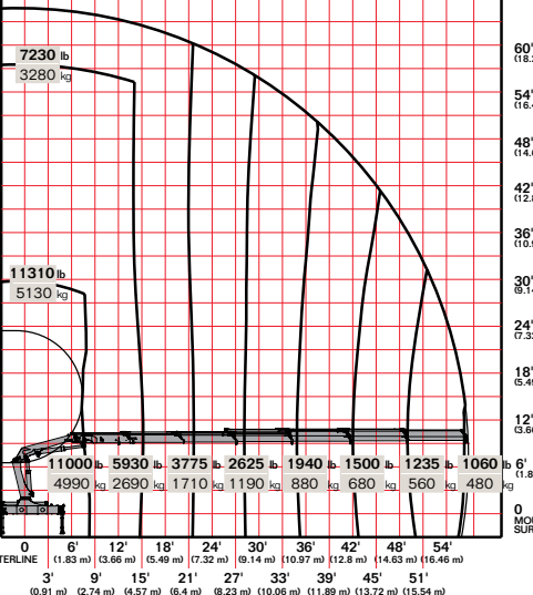
15/105DL K6
