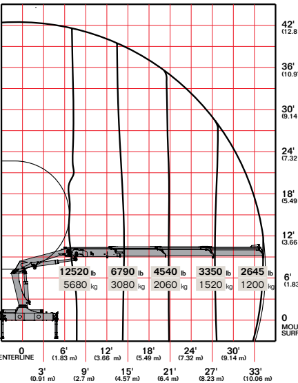
15/105DL K5
