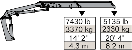
15/105DL - 2 Hydraulic
