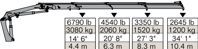
15/105DL - 3 Hydraulic
