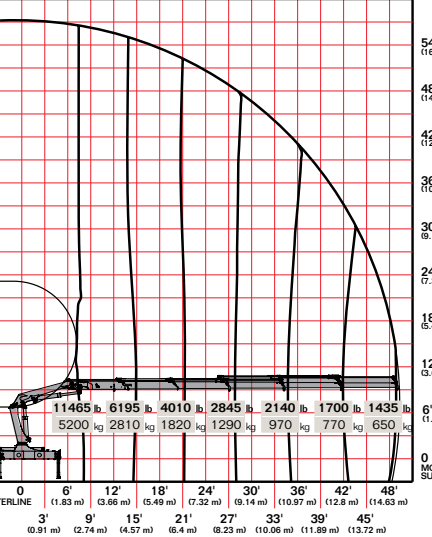
15/105DL K5
