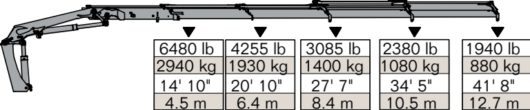
15/105DL - 4 Hydraulic
