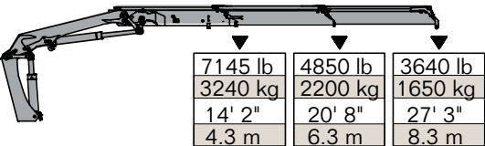
15/105DL - 3 Hydraulic
