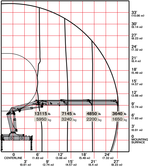
15/105DL K2
