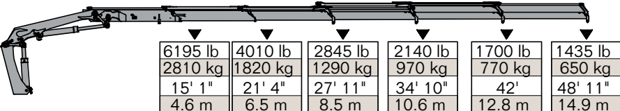
15/105DL - 5 Hydraulic
