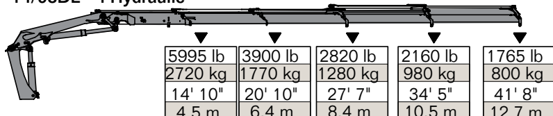
14/98DL - 5 Hydraulic
