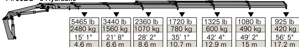
14/98DL - 6 Hydraulic
