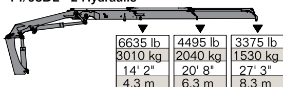
14/98DL - 3 Hydraulic
