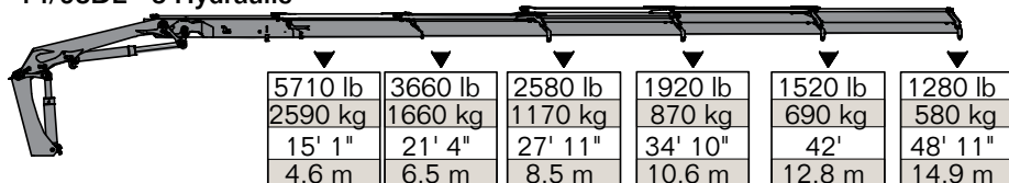
14/98DL - 6 Hydraulic
