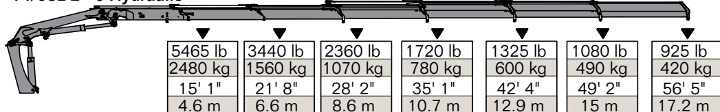
14/98DL - 6 Hydraulic
