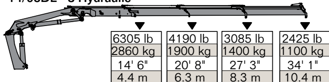
14/98DL - 4 Hydraulic
