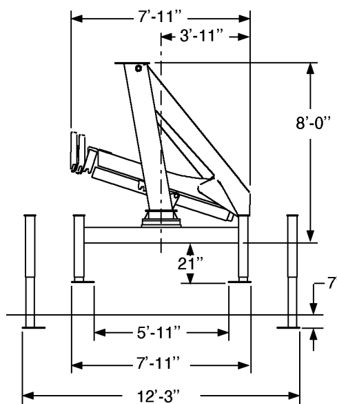
STOWED POSITION & OUTRIGGER DIMENSIONS
